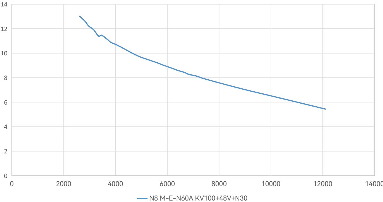
Thrust-Efficiency Curve
