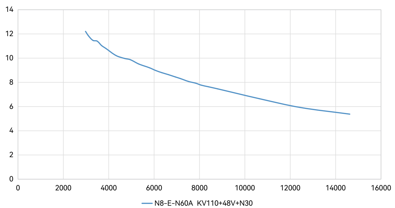
Thrust-Efficiency Curve
